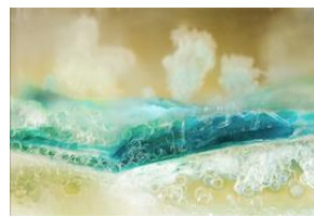
Subduction Zone
